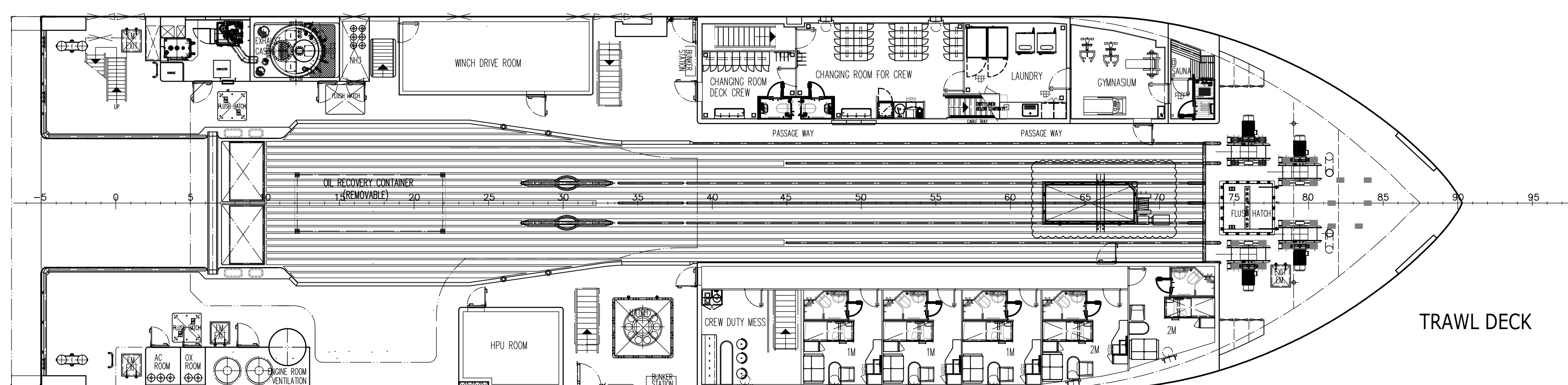
1st. DECK
