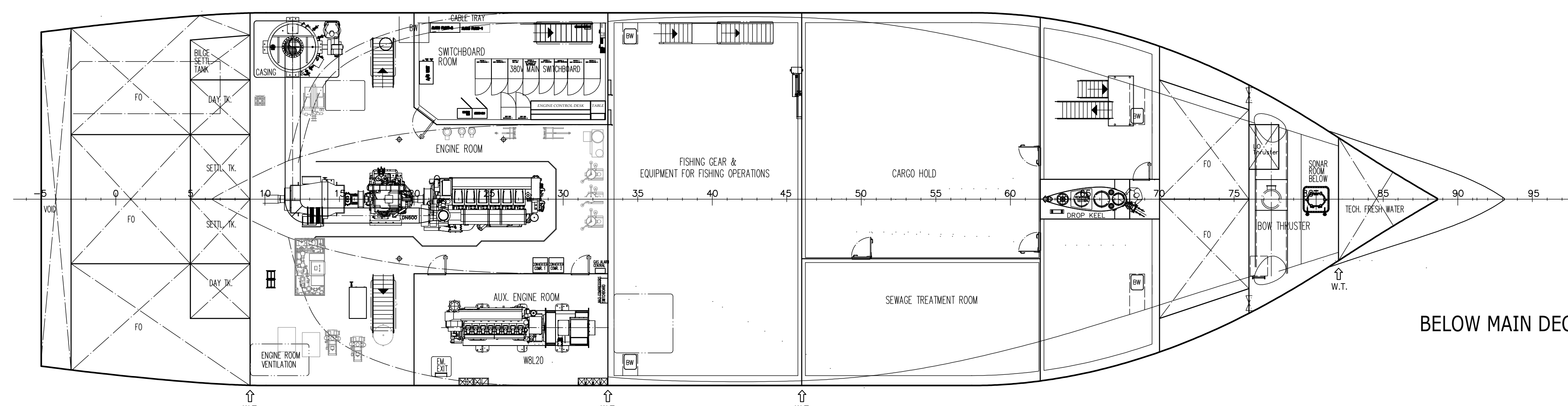
MAIN DECK
