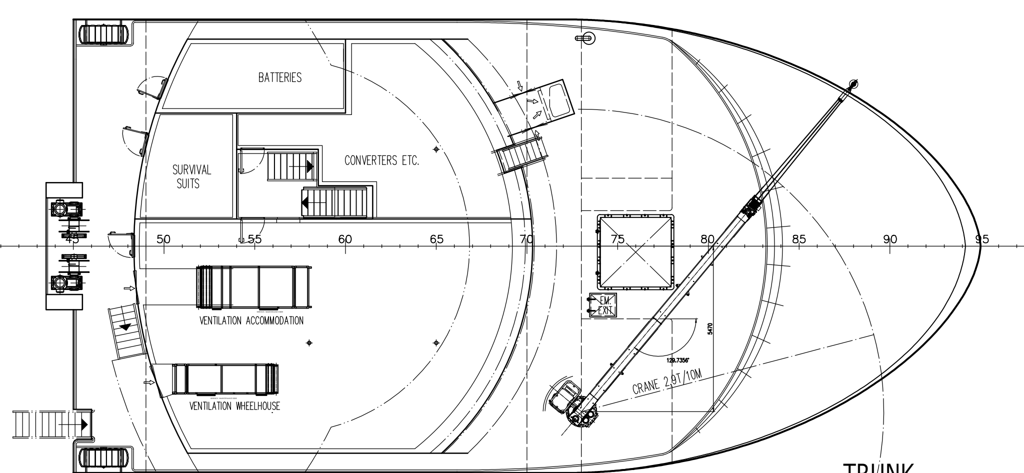
TRUNK
