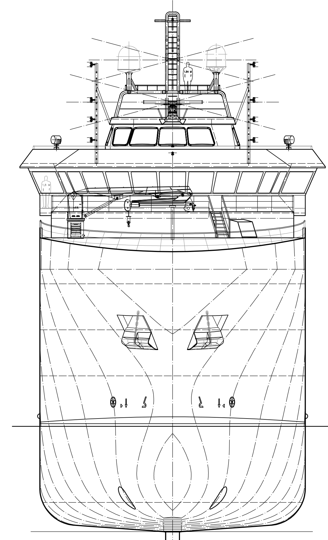
FRONT VIEW
