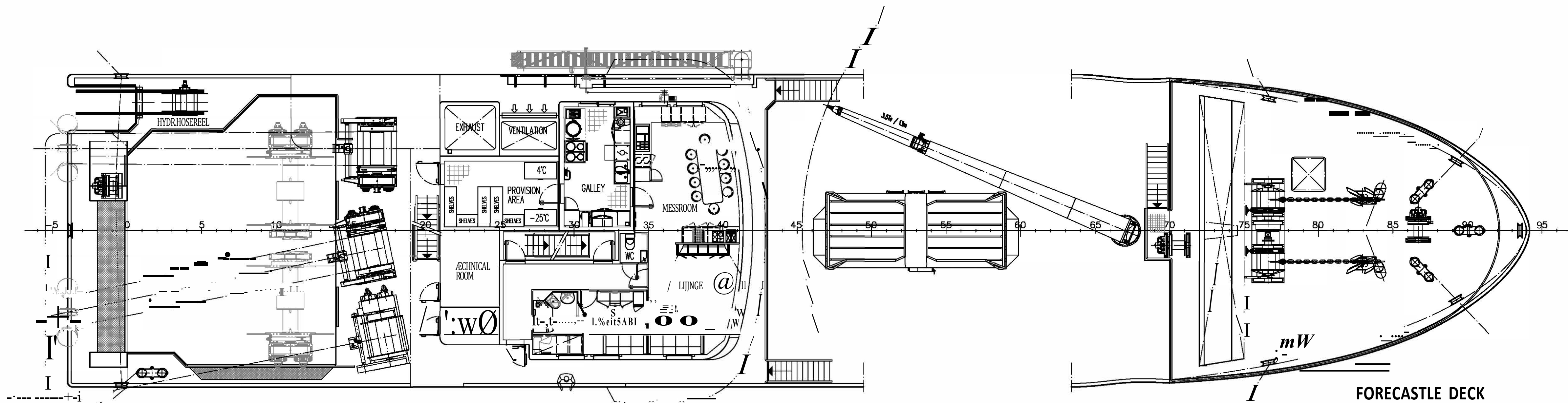
FORECASTLE DECK
